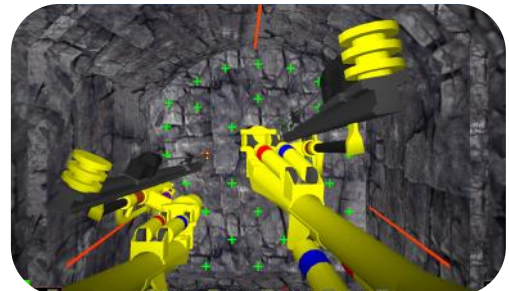
Drilling a complete round using two booms, grade and back line orientation cues
