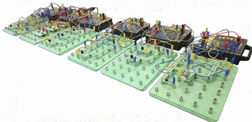
Automotive CANbus W/ Gateway Module Trainer (p. 3)
