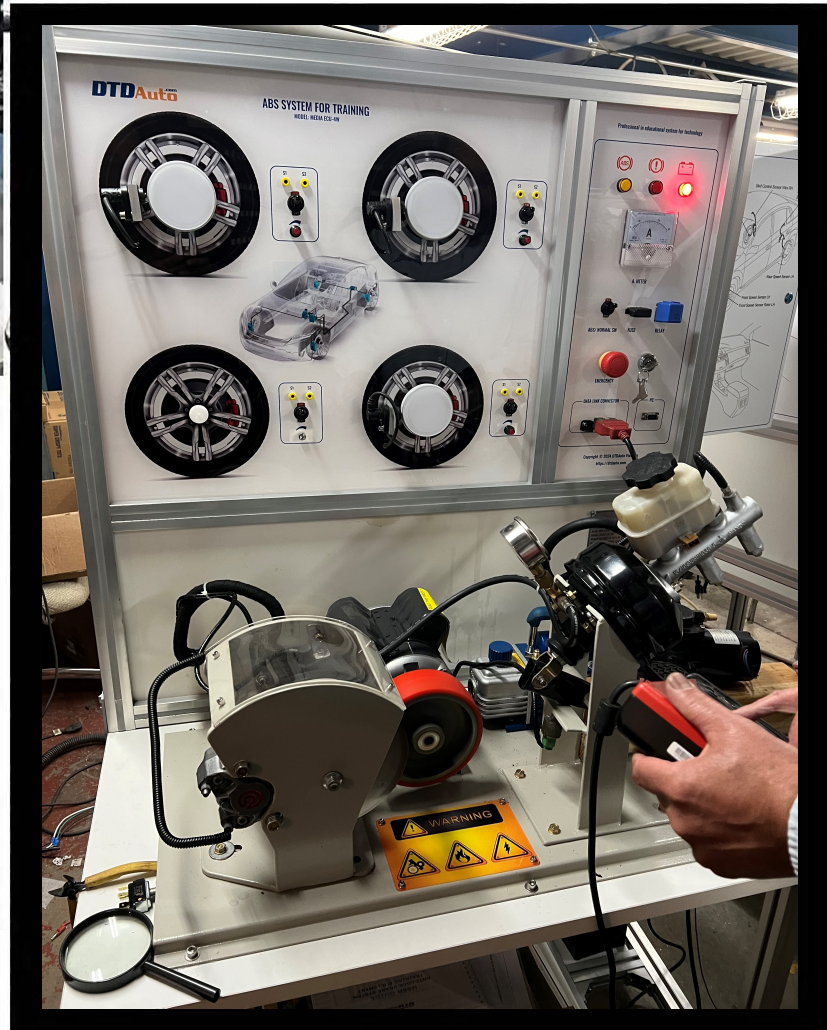
Four Wheel ABS Trainer
