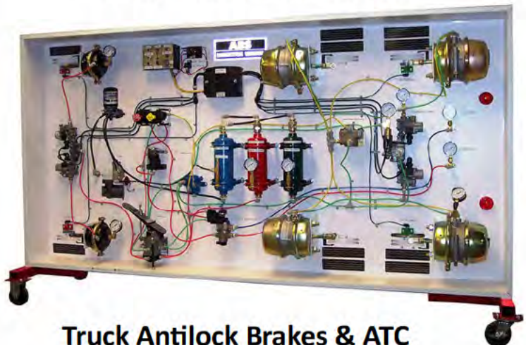
Truck Brake Lab at Pikes Peak Community College
